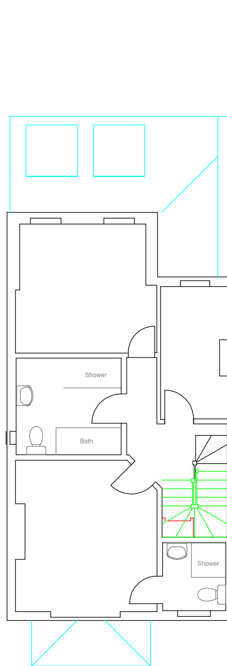
First Floor and Roof
