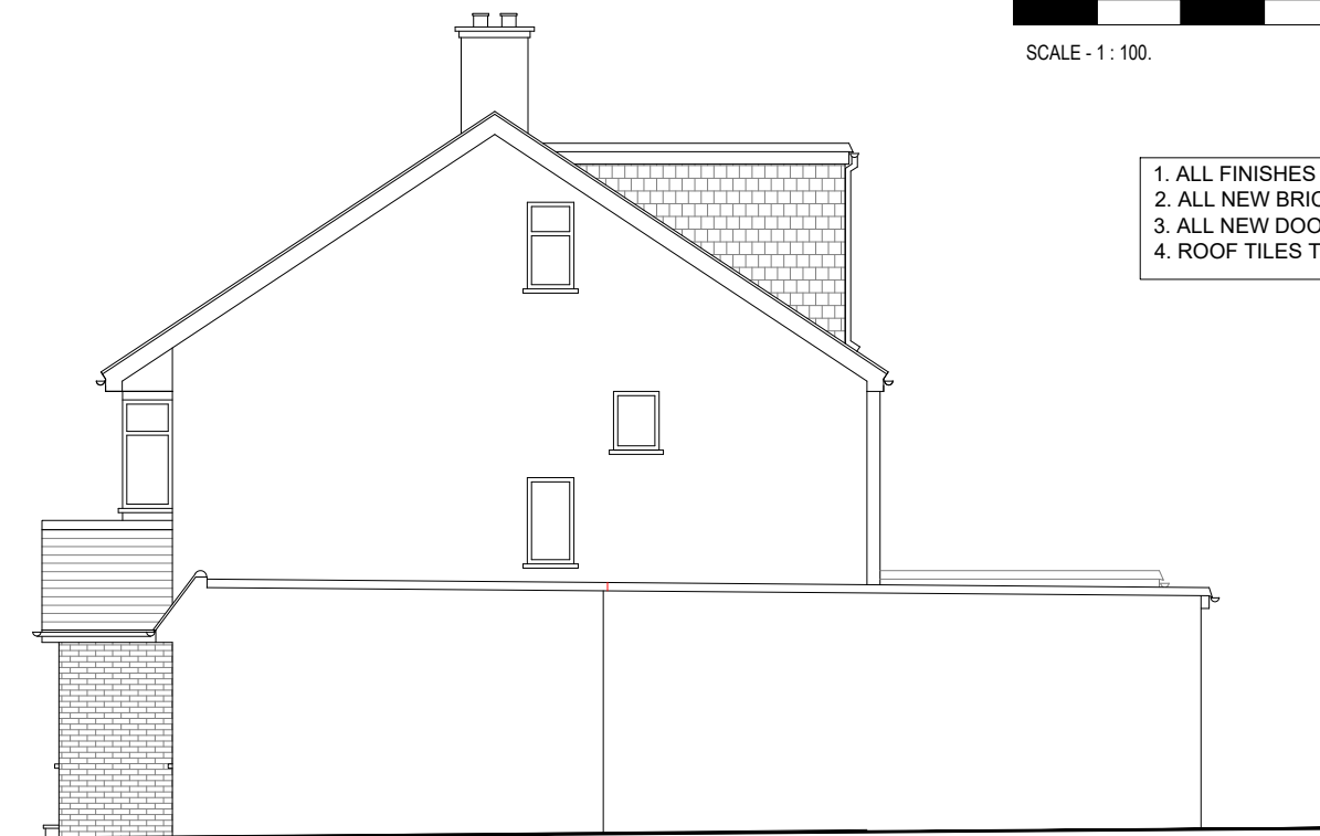
EXISTING RIGHT ELEVATION
