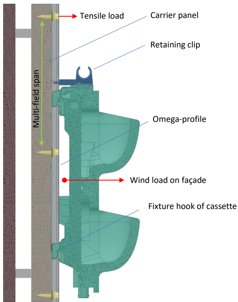
Figure 1 – Schematic representation of fixture of MobiPanel on a carrier panel
