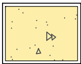
SELF BINDING GRAVEL FOOTPATH To be surfaced dressed with Breedon self binding gravel wearing course. To be edged with PCC edgings 915x50x150mm. Geotextile to be installed beneath sub base.
