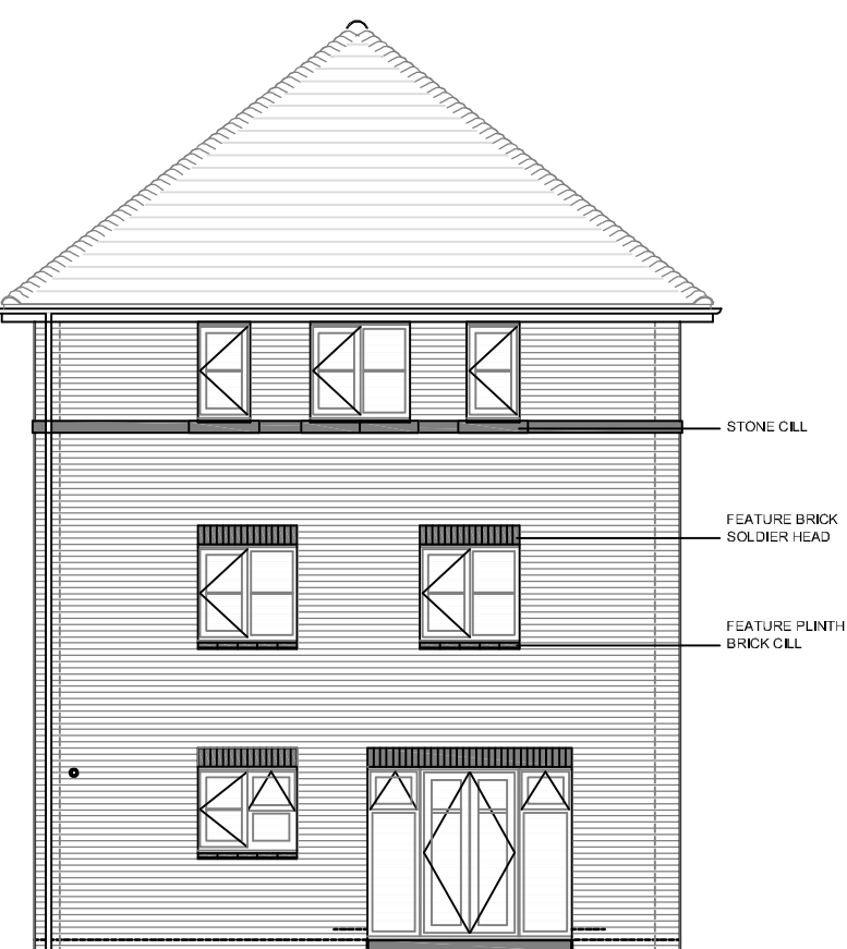
TYPICAL REAR ELEVATION HOUSE TYPE U
