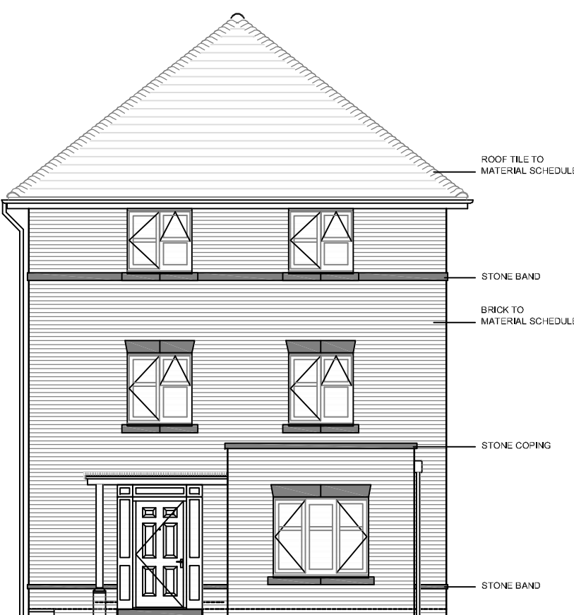
TYPICAL FRONT ELEVATION HOUSE TYPE U
