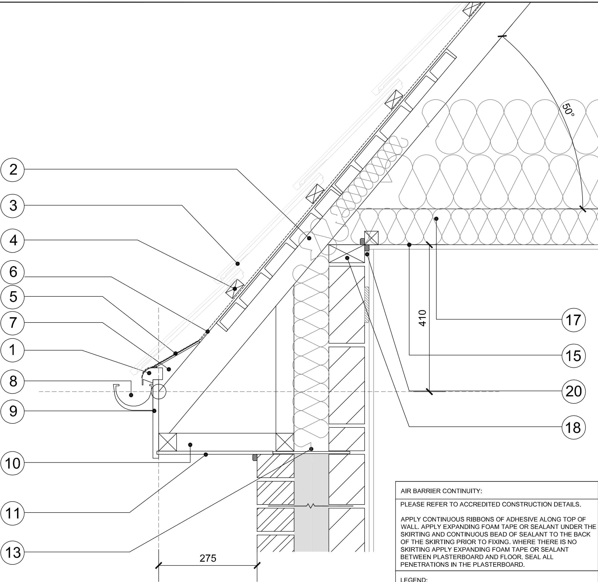
BOXED EAVES DETAIL 50° TYPE Y
