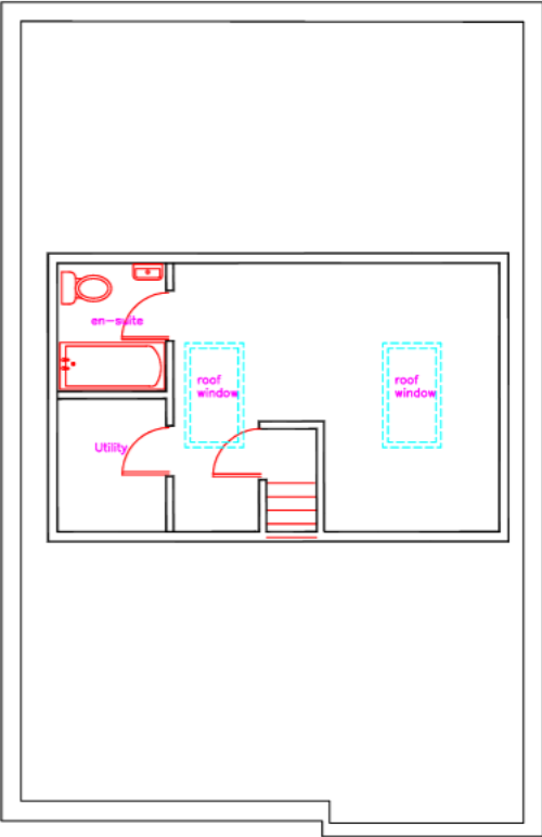
Second floor plan 1:100
