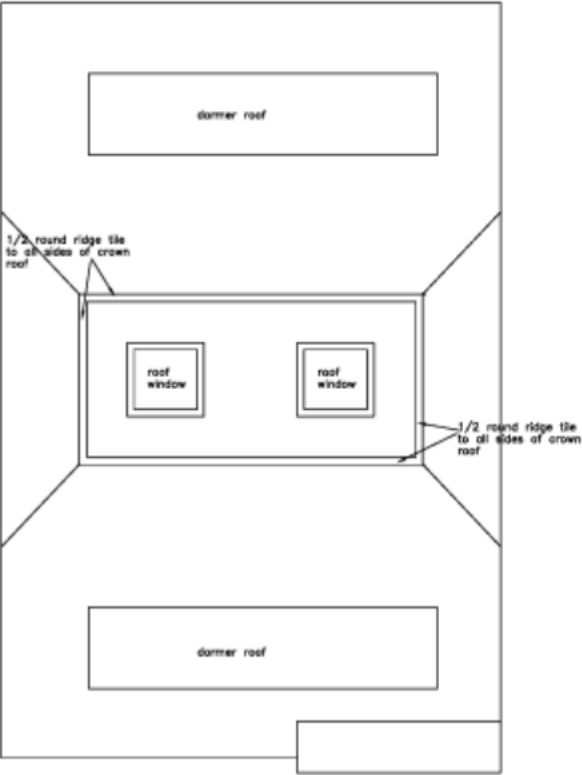
Roof plan 1:100 as proposed
