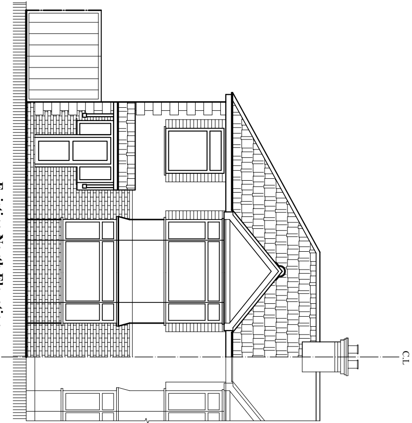
Existing North Elevation
