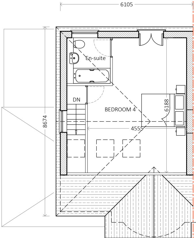
ROOF PLAN
