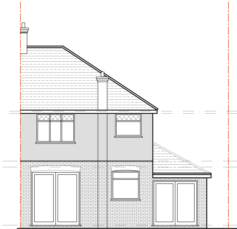
REAR ELEVATION
