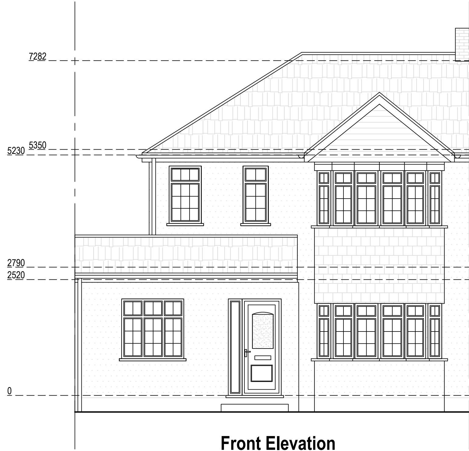
Front Elevation
