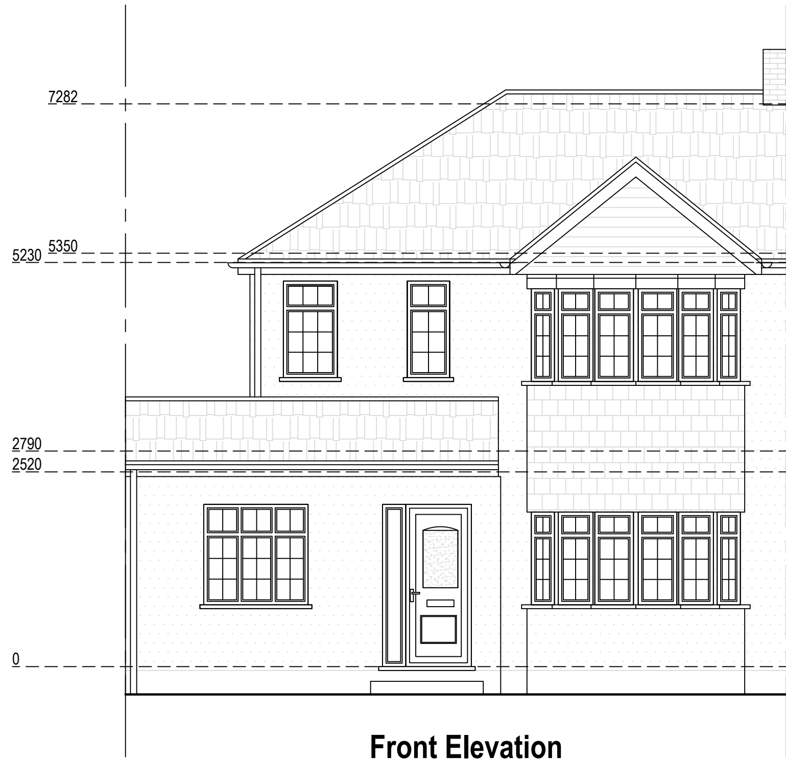
Front Elevation
