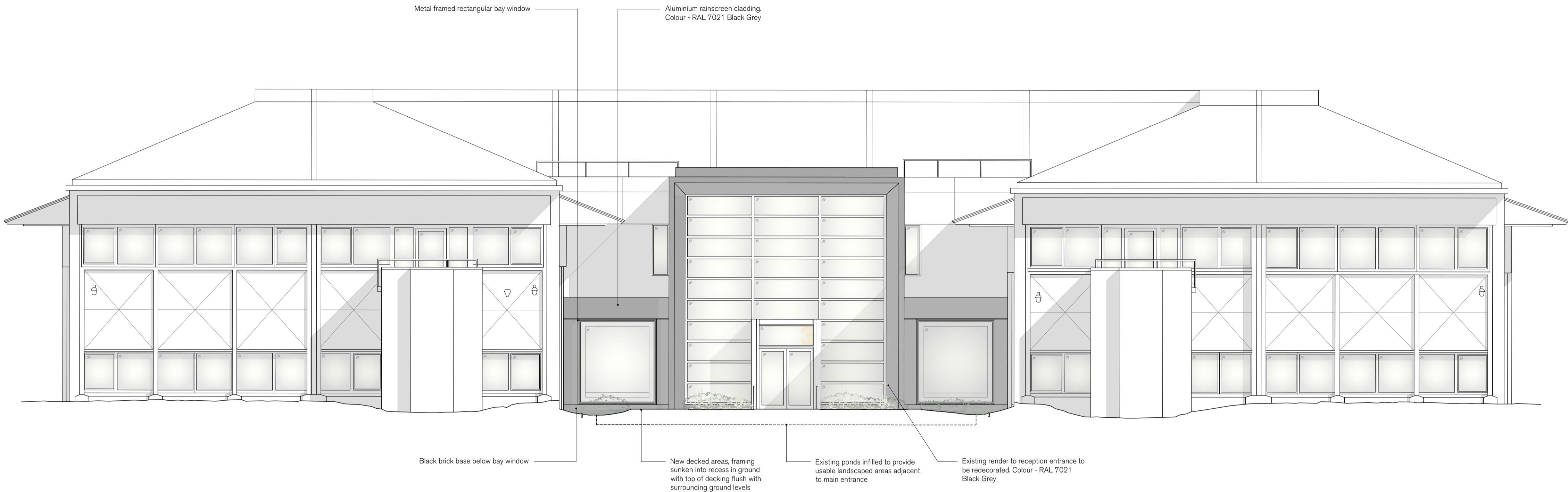
PROPOSED EAST ELEVATION 01 1:100
