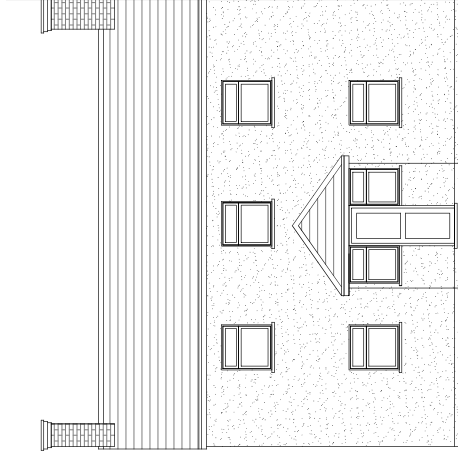
Existing Front Elevation Scale 1:100
