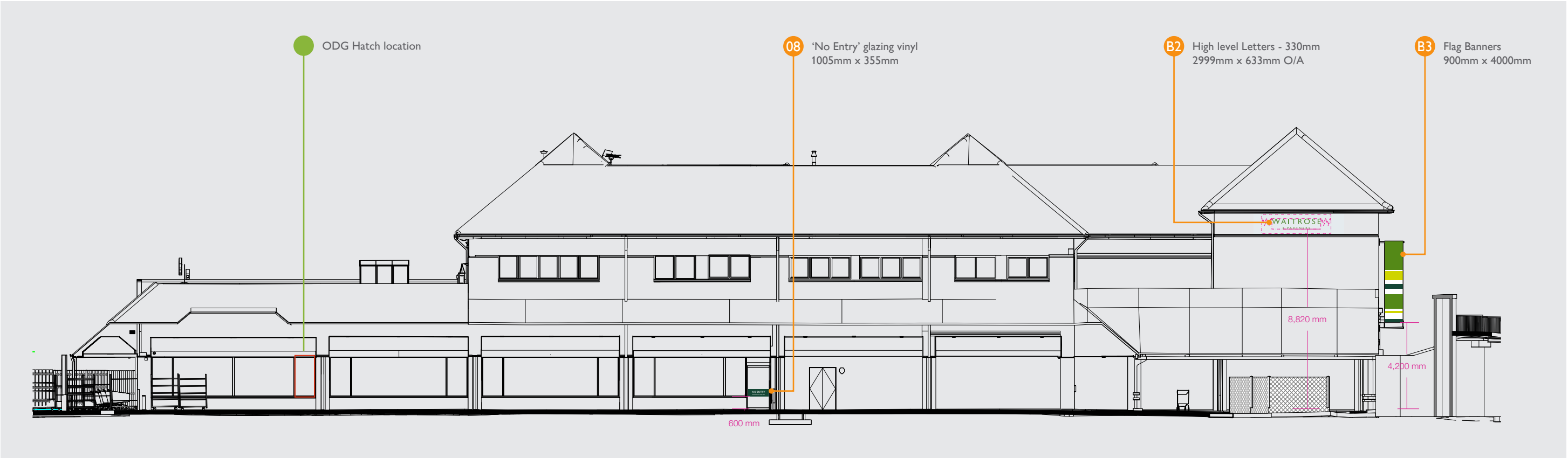
B Proposed South Elevation
