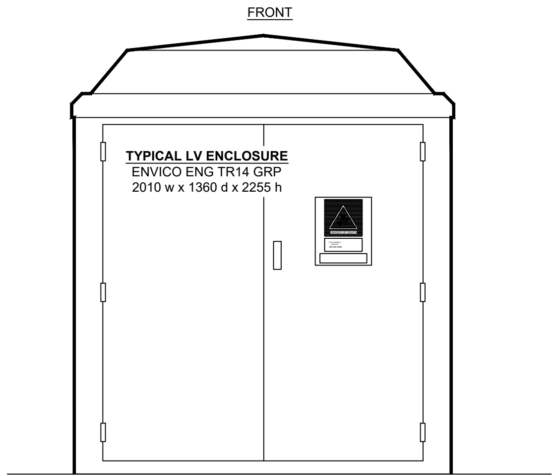
Elevation A Scale 1:20
