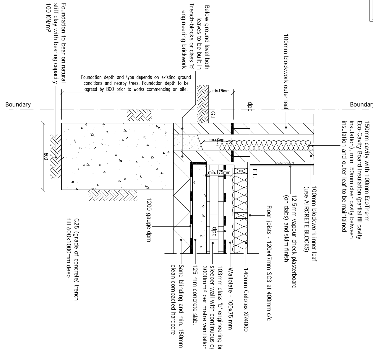
FOUNDATION DETAIL ON BOUNDARY scale 1:20
