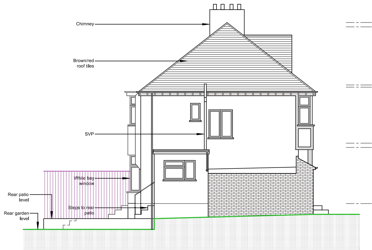
EXISTING SIDE ELEVATION (LHS)
