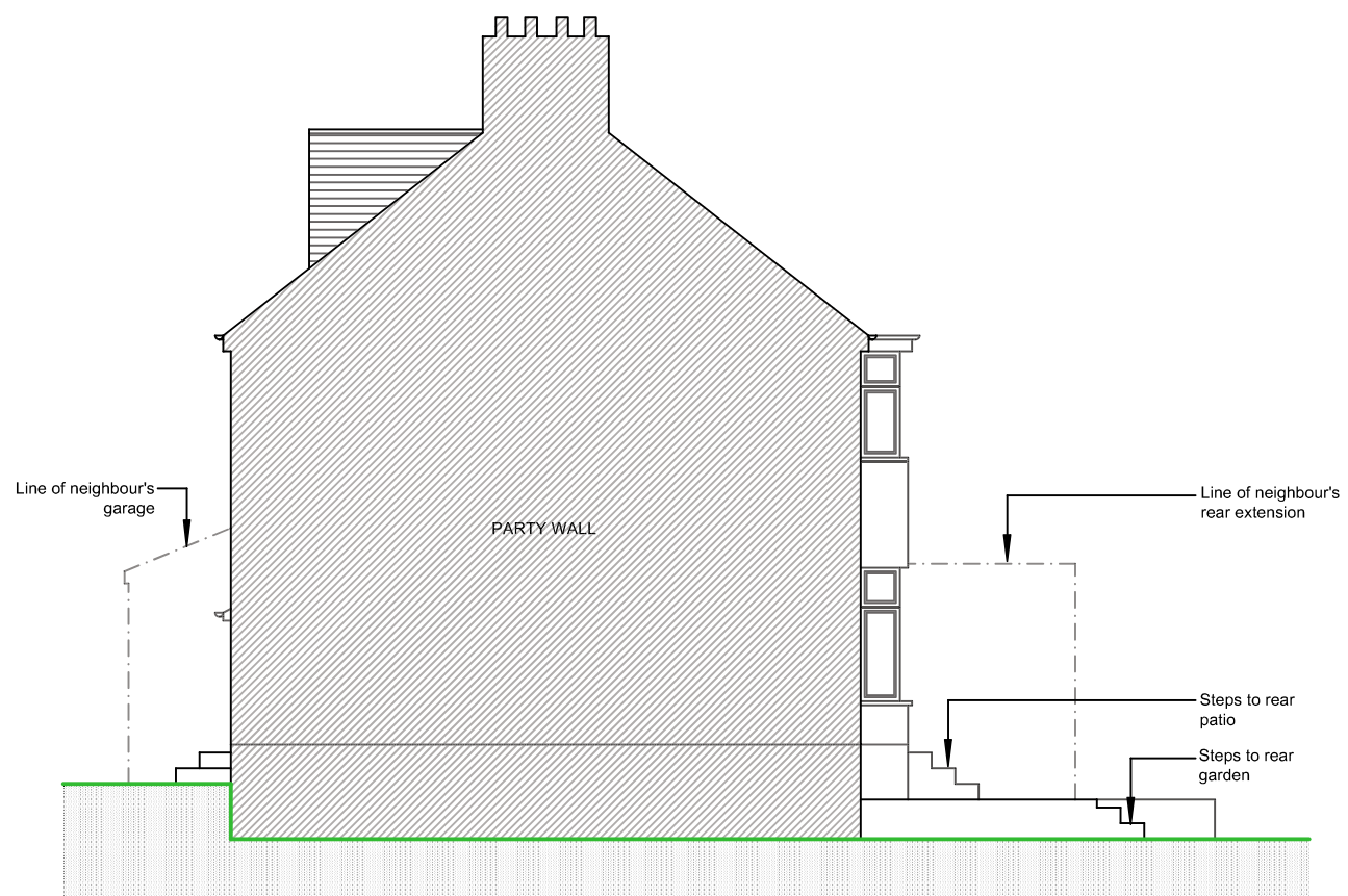
EXISTING SIDE ELEVATION (RHS)
