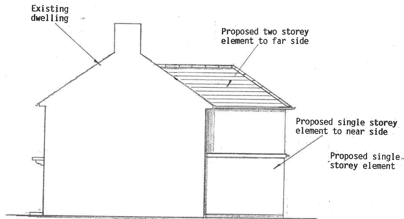
PROPOSED FLANK ELEVATION (FROM N° 6) 1:100
