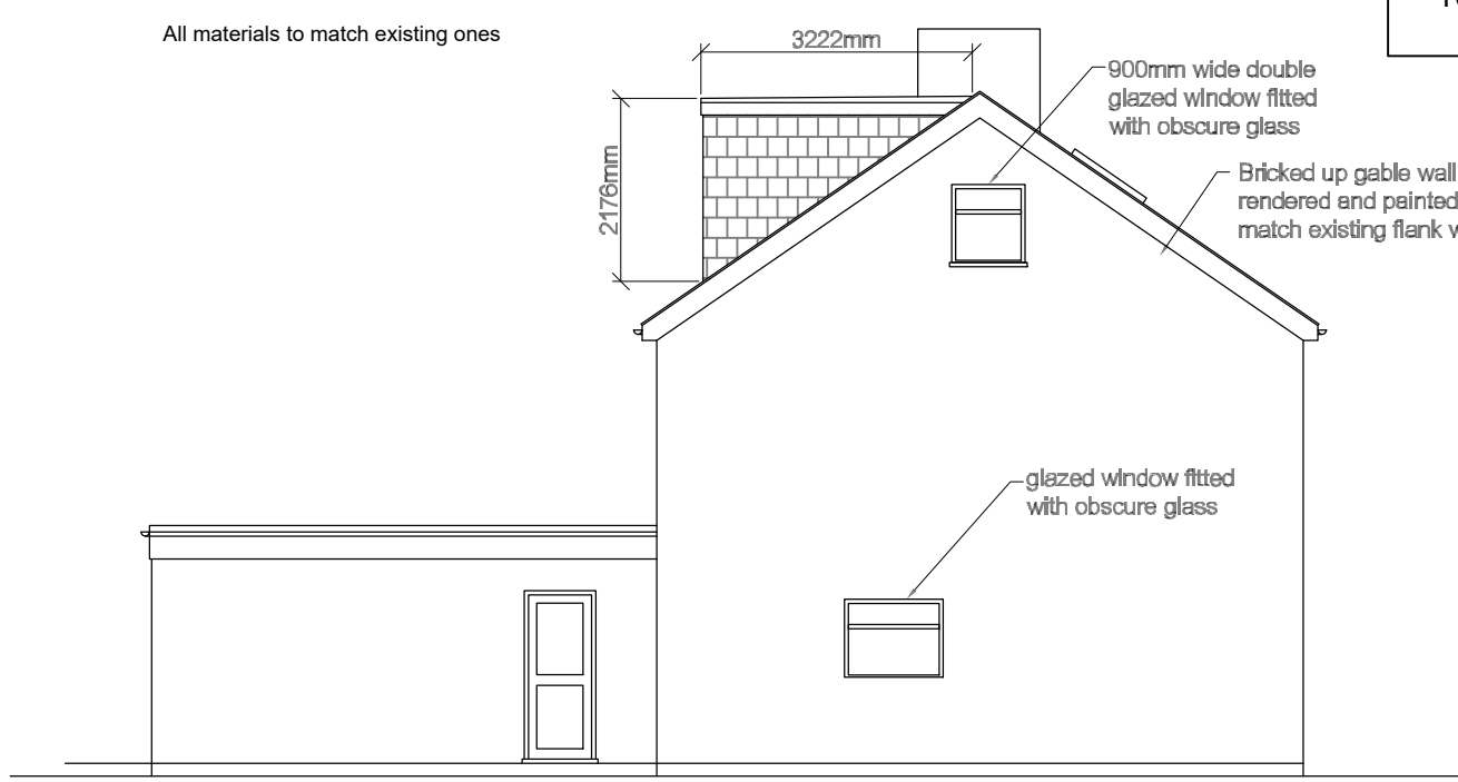
PROPOSED SIDE ELEVATION ESC.: 1/100
