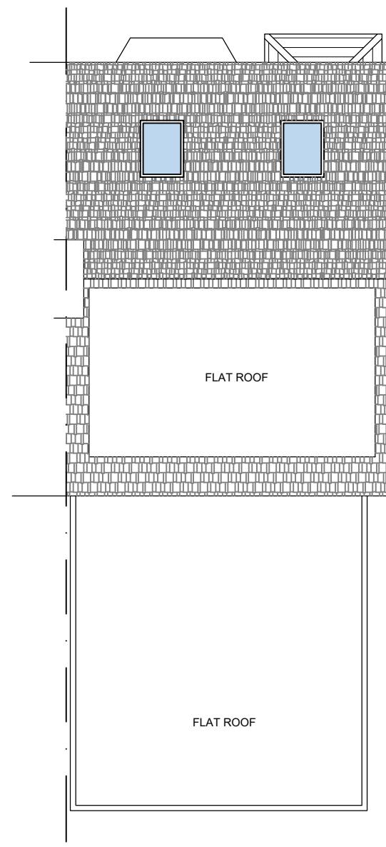
PROPOSED ROOF PLAN ESC.: 1/100
