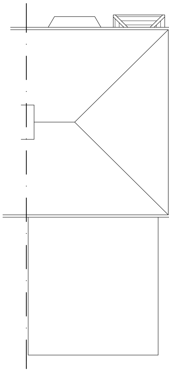
EXISTING ROOF PLAN ESC.: 1/100
