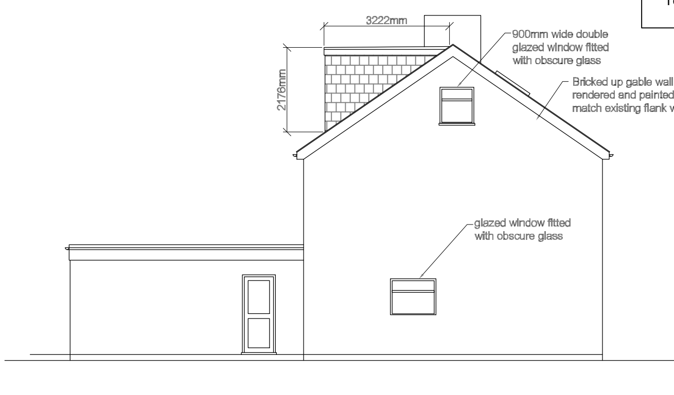
PROPOSED SIDE ELEVATION ESC.: 1/100
