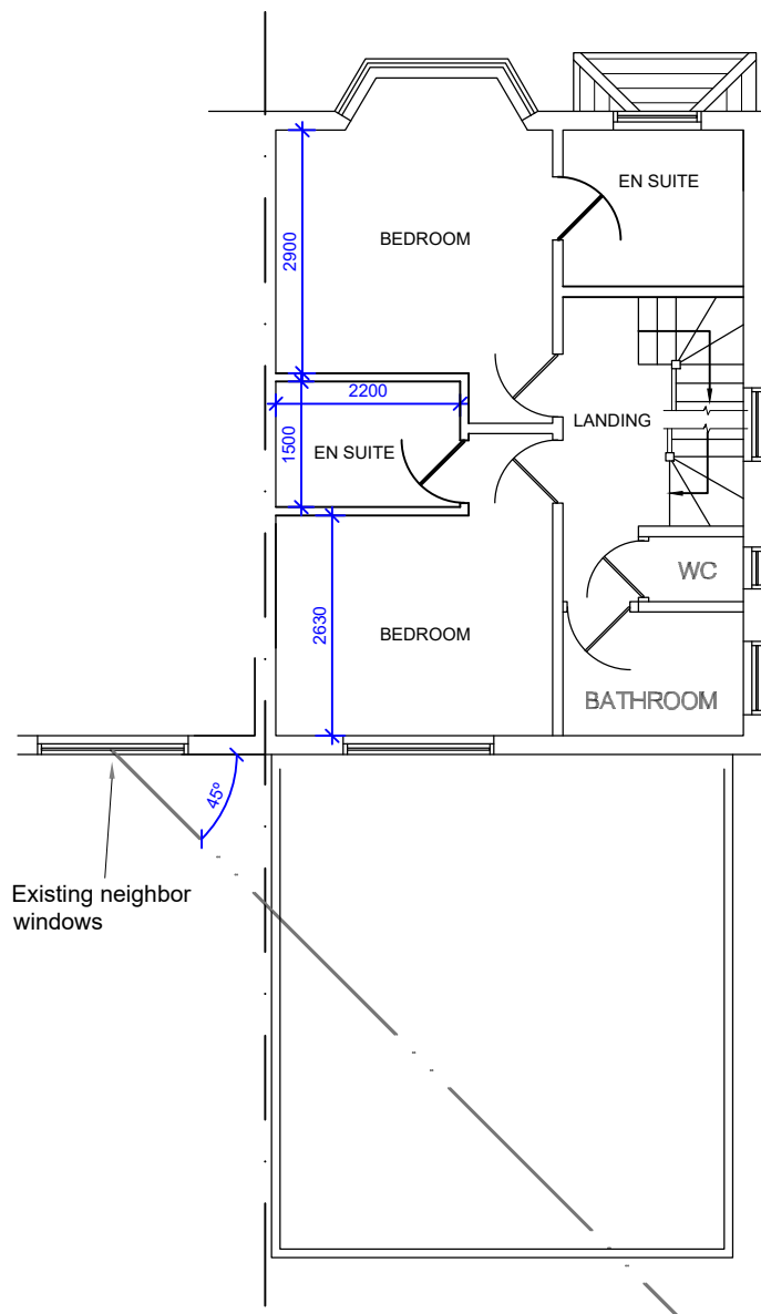
PROPOSED FIRST FLOOR ESC.: 1/100
