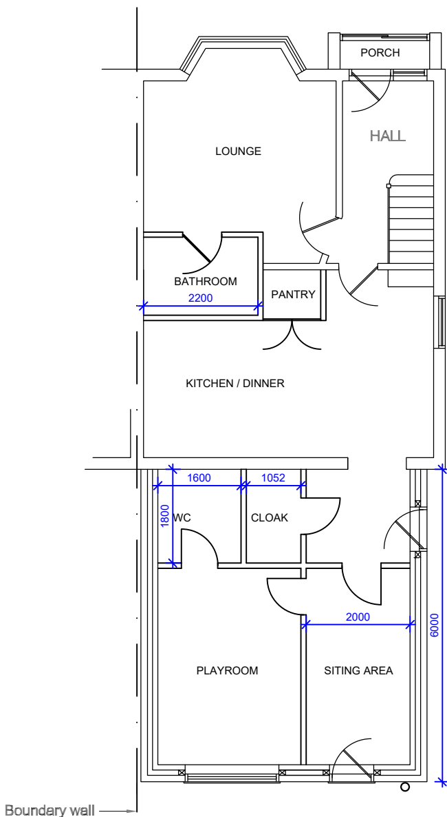
PROPOSED GROUND FLOOR ESC.: 1/100
