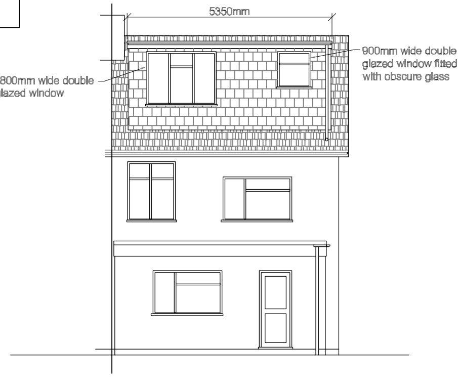
PROPOSED REAR ELEVATION ESC.: 1/100
