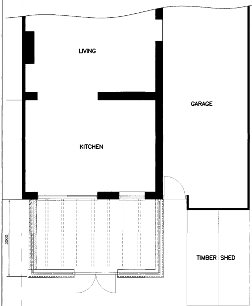
PROPOSED PART GROUND FLOOR PLAN
