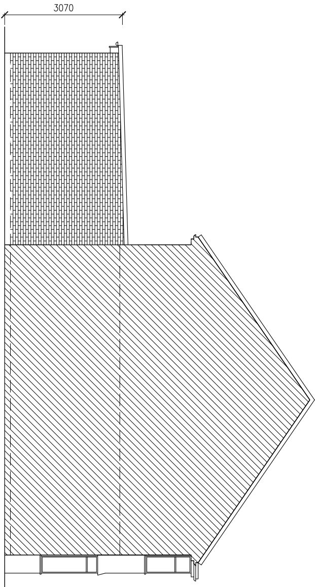
PROPOSED LEFT SIDE ELEVATION (SECTIONAL) 1:100
