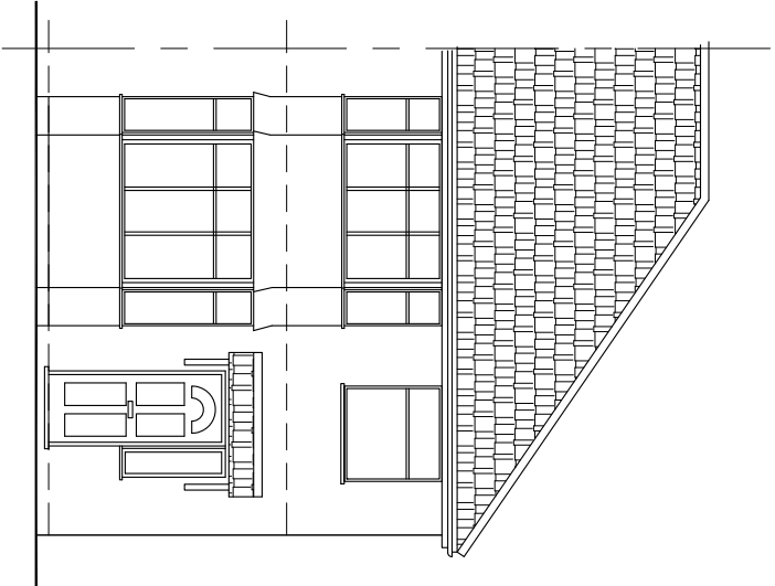
EXISTING FRONT ELEVATION 1:100 (NO CHANGE)
