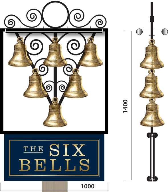
ITEM A. ONE NEW DOUBLE SIDED PICTORIALTO EXISTING POST. WITH NEW LINOLITS HIEGHT ABOVE GROUND 3M
