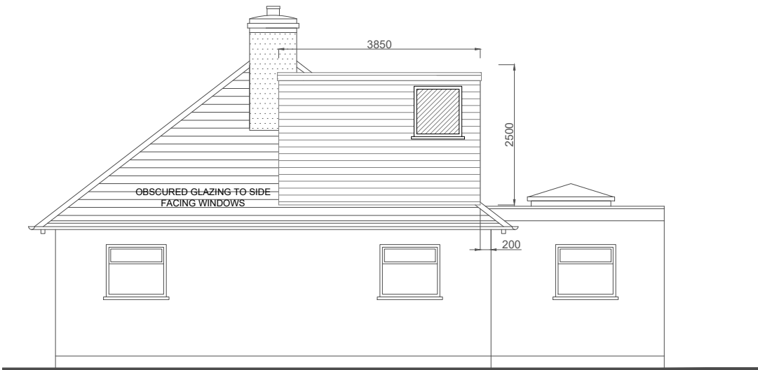
South Elevation As Proposed
