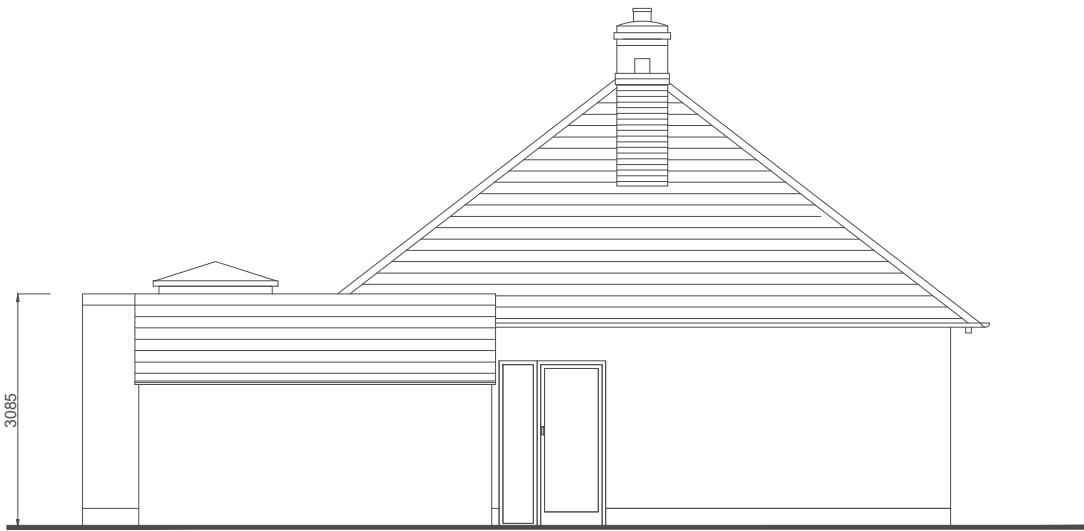
North Elevation As Existing
