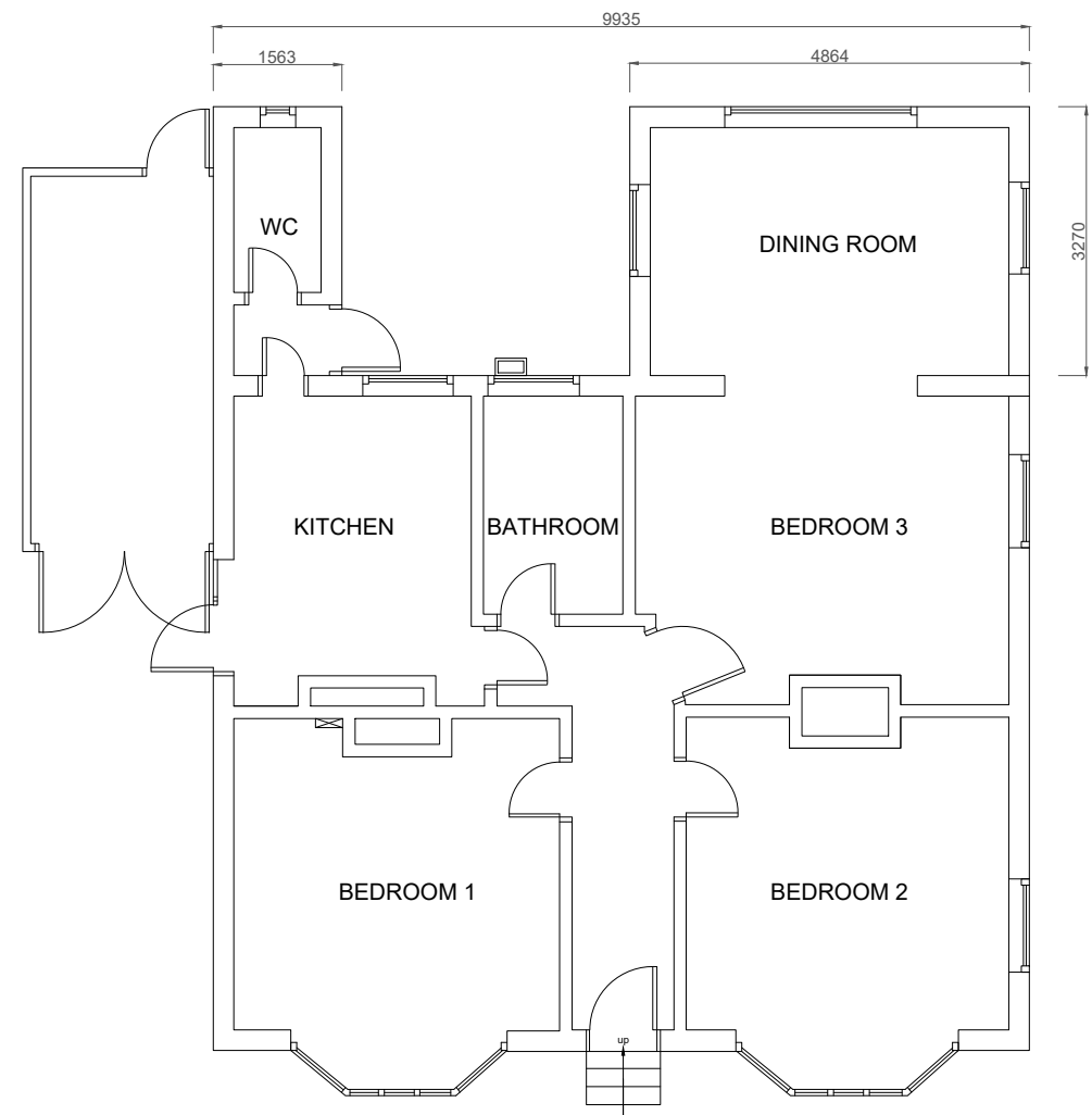
Ground Floor Plan As Pre-Existing
