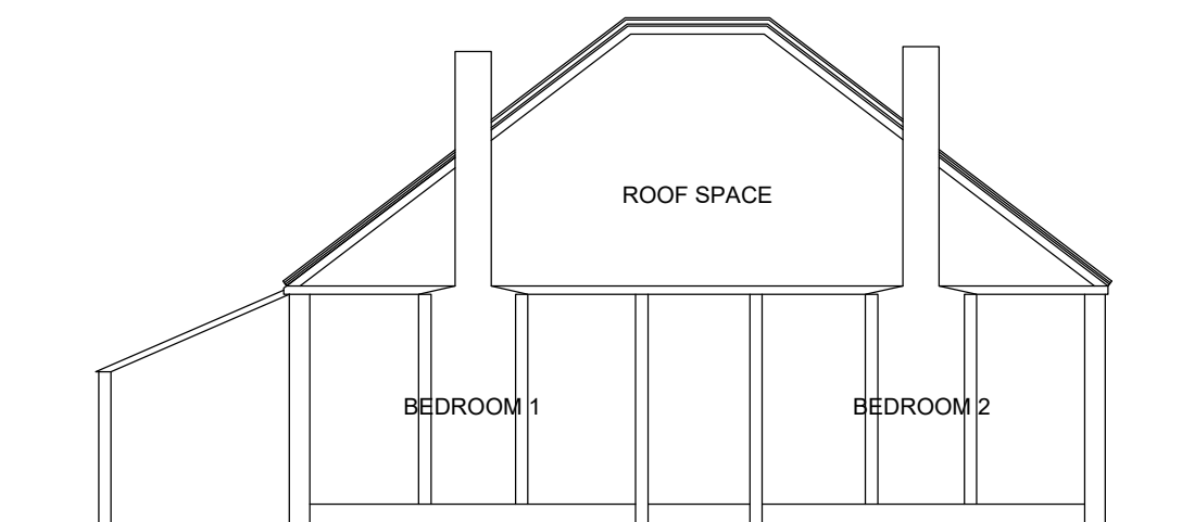
Section X As Pre-Existing 0 5m scale
