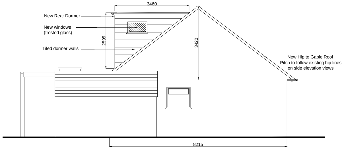
North Elevation As Proposed
