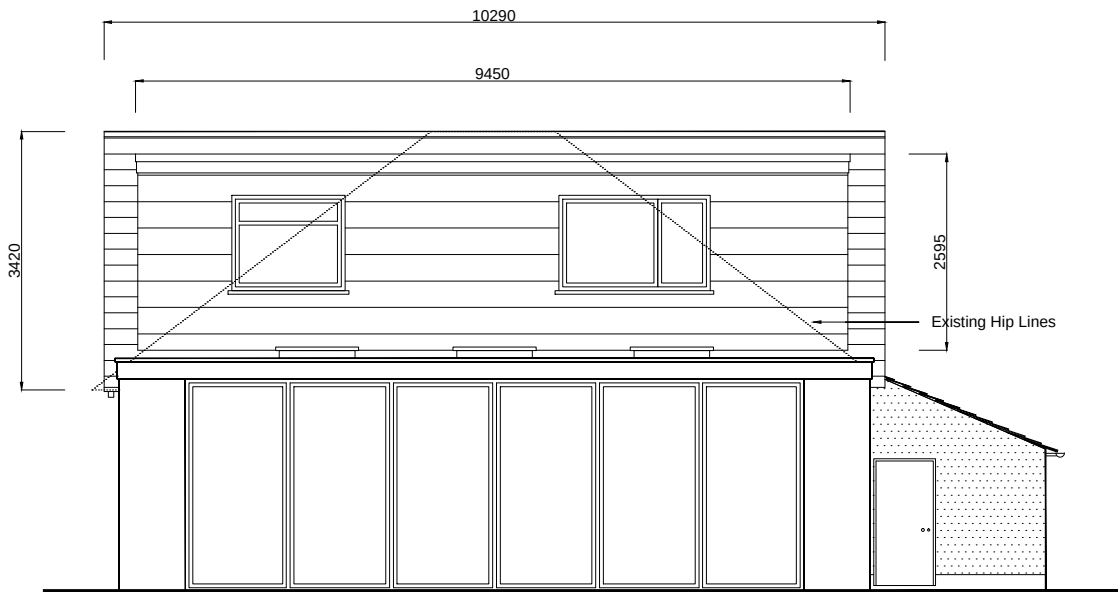
East Elevation As Proposed
