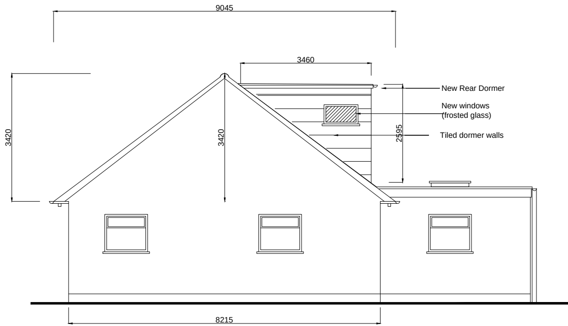
South Elevation As Proposed
