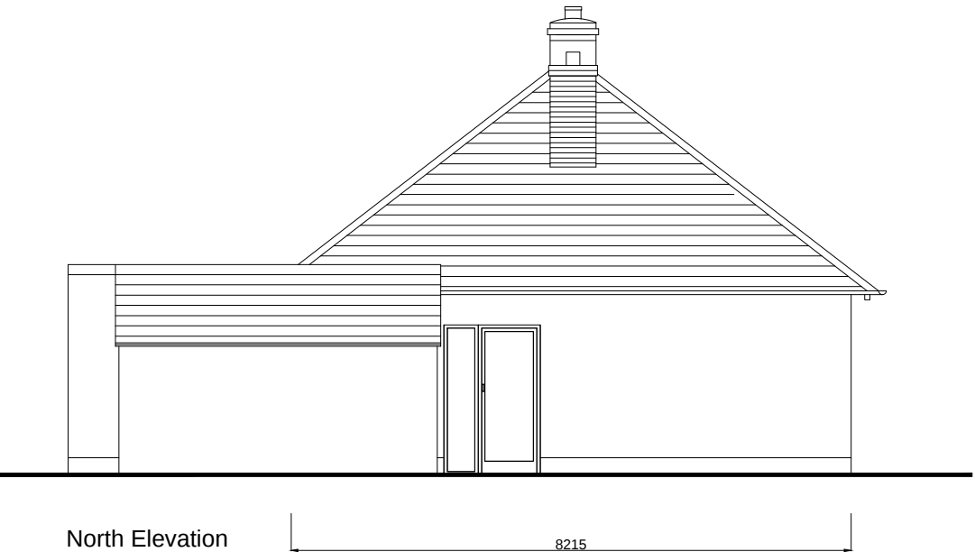
North Elevation As Existing
