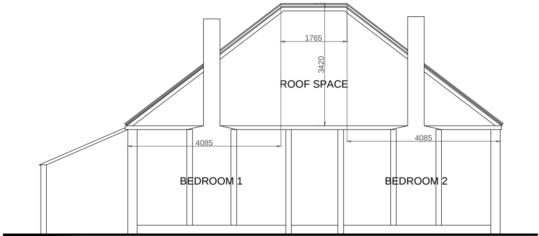
Section X As Existing
