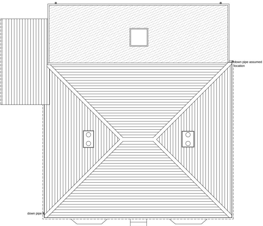
Roof Plan As Existing
