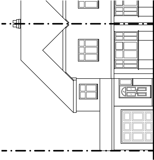
EXISTING FRONT (SOUTH-EAST) ELEVATION
