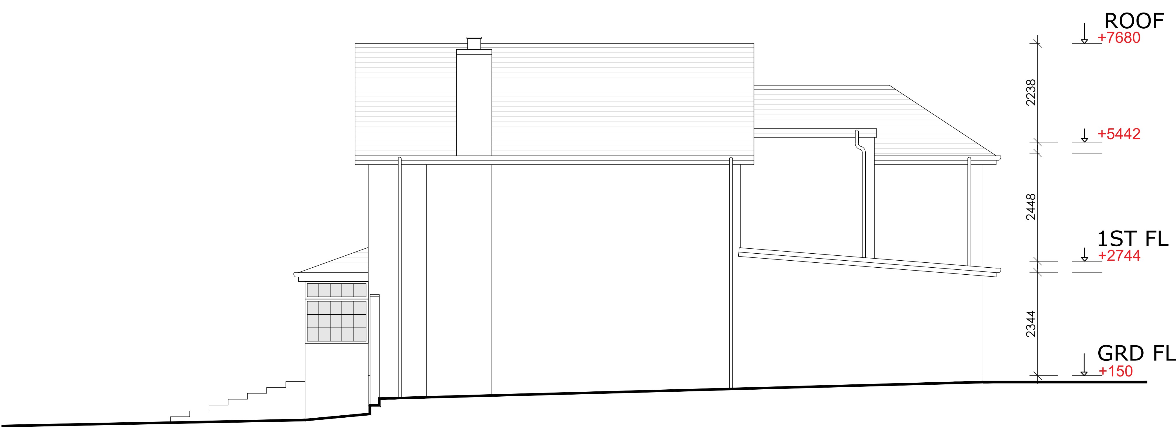
PROPOSED SIDE ELEVATION
