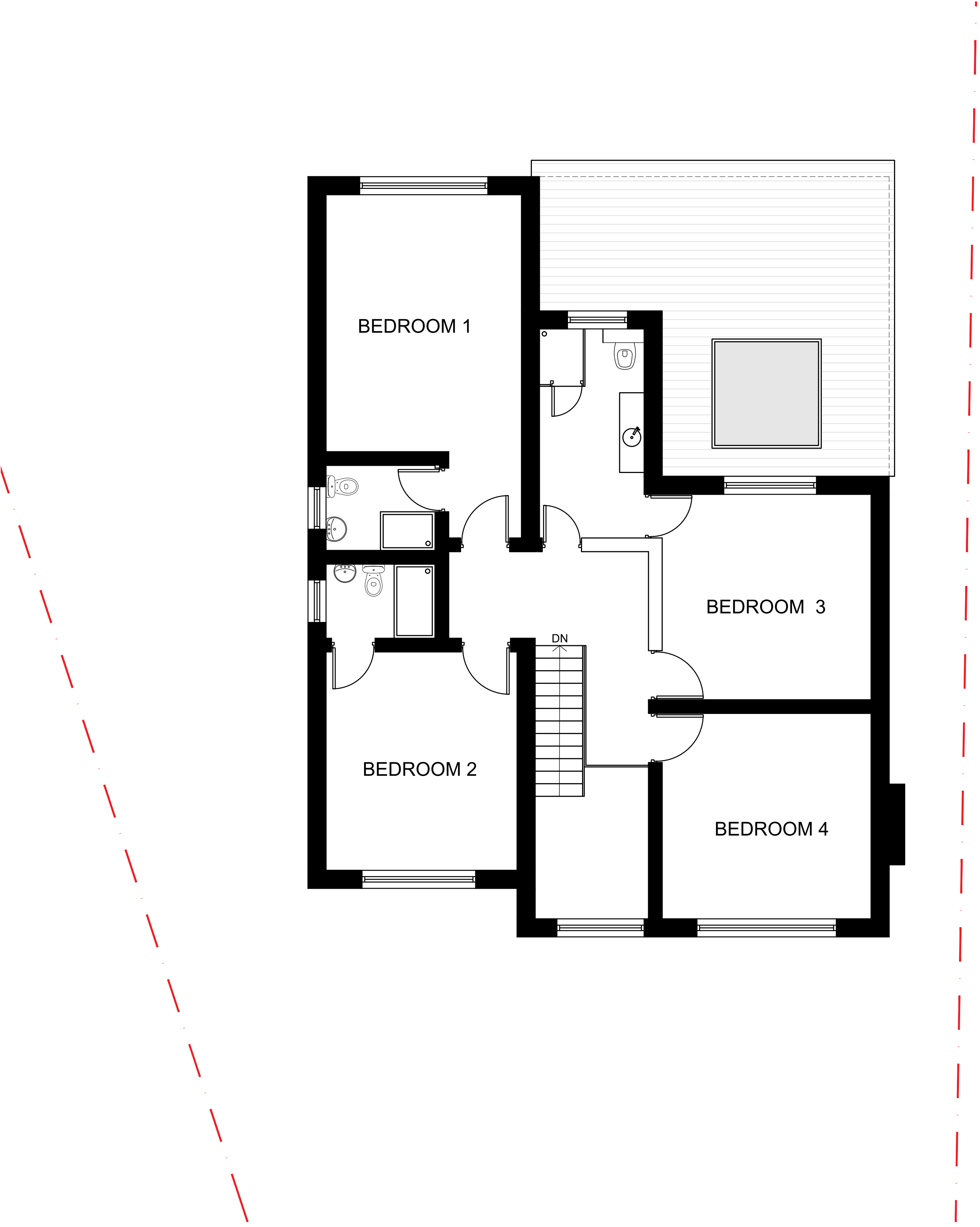
EXISTING FIRST FLOOR
