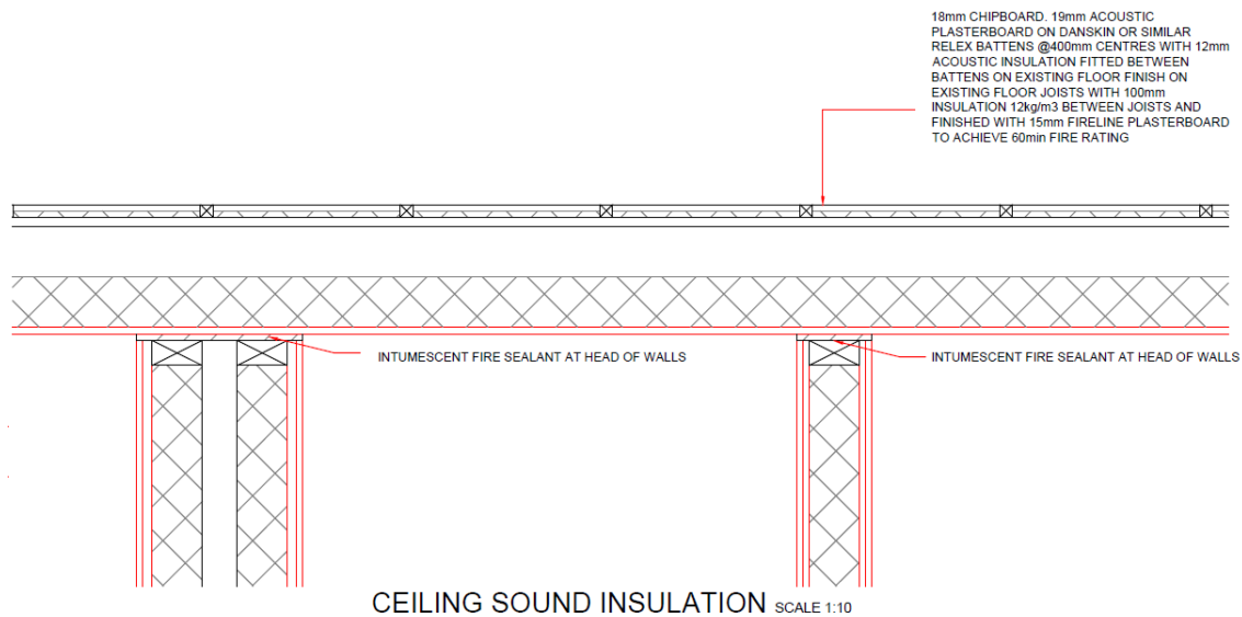
Figure 2: Suggested ceiling scheme for additional sound insulation for the floor between ground floor rooms and upper floor rooms.
