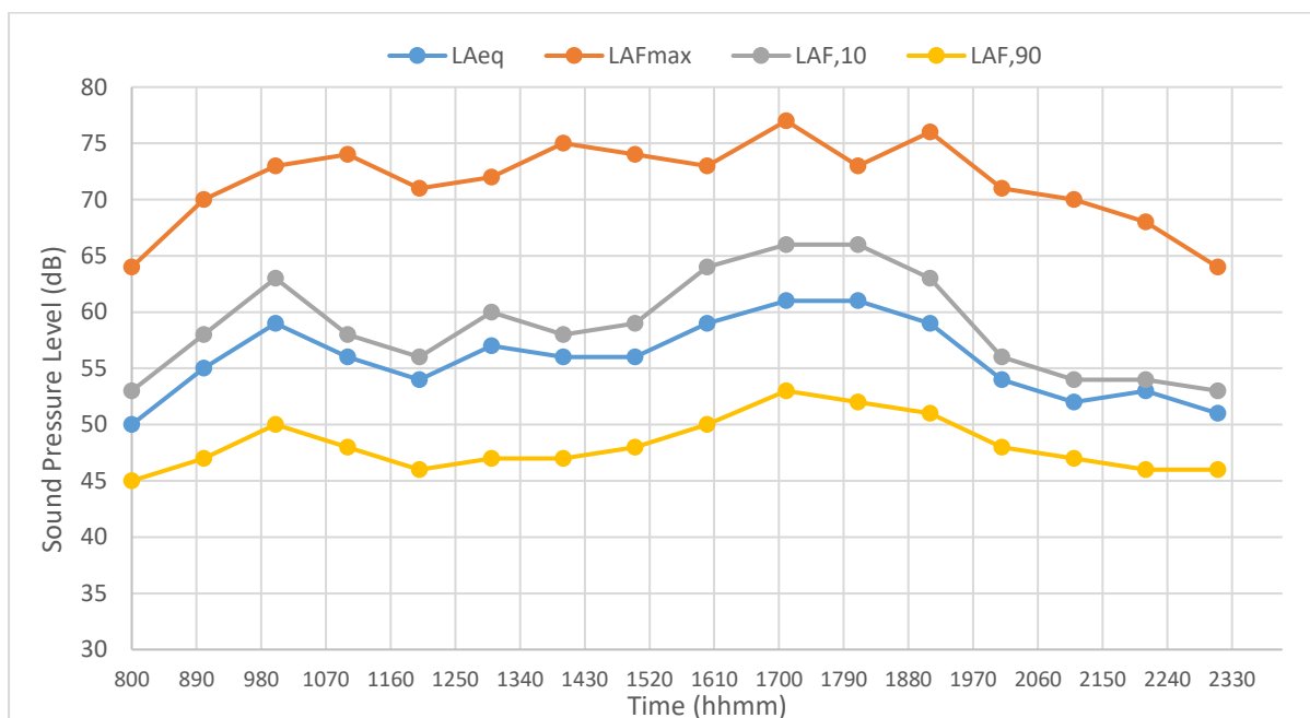
Figure 1: A graphical comparison of the noise indices at the site for the daytime 16-hours on.
