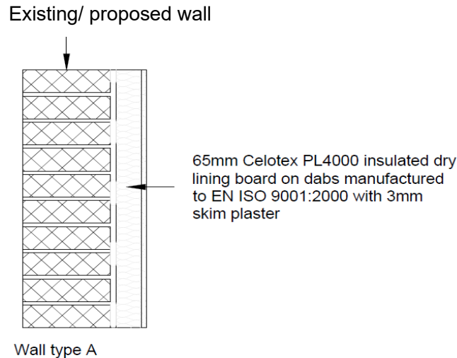
Figure 4: Upgrade of insulation to external walls of the rooms.
