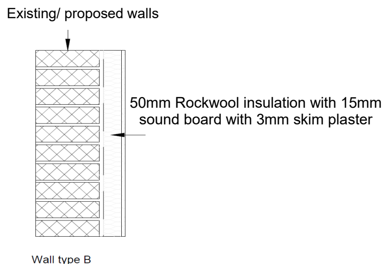
Figure 3: Upgrade of insulation to the party wall of the rooms.
