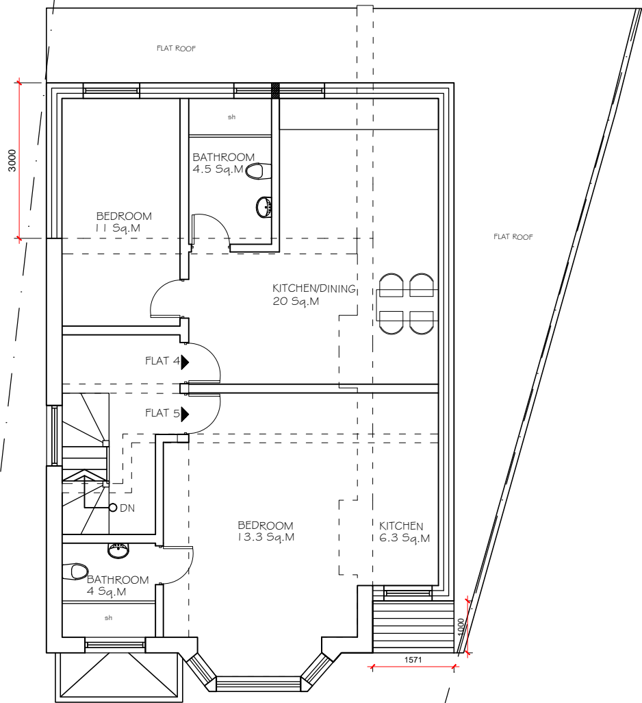
PROPOSED FIRST FLOOR PLAN (Existing flats enlarged through extensions)
