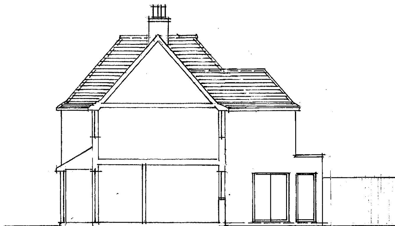
Proposed Side Elevation (South)
