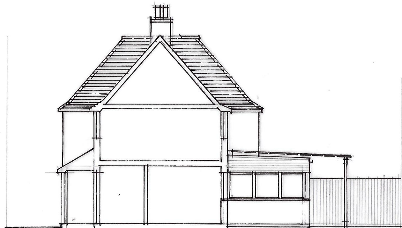
Existing Section / Side Elevation (South)
