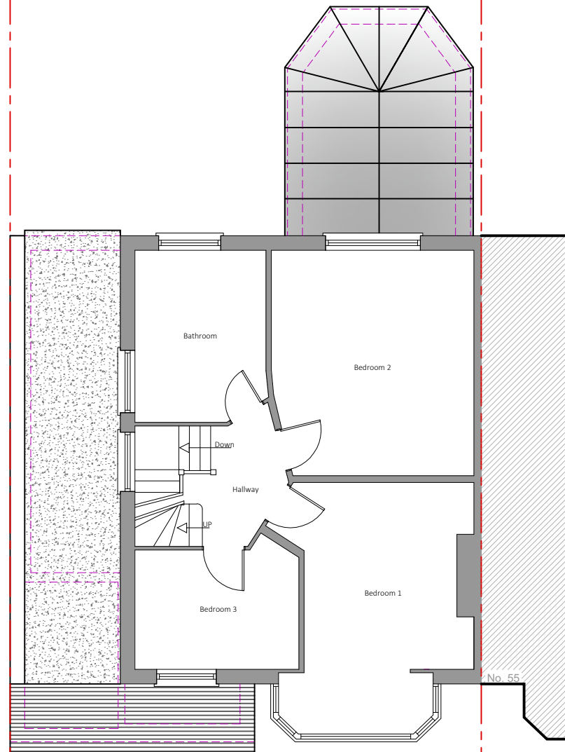
2 Existing First Floor Plan
