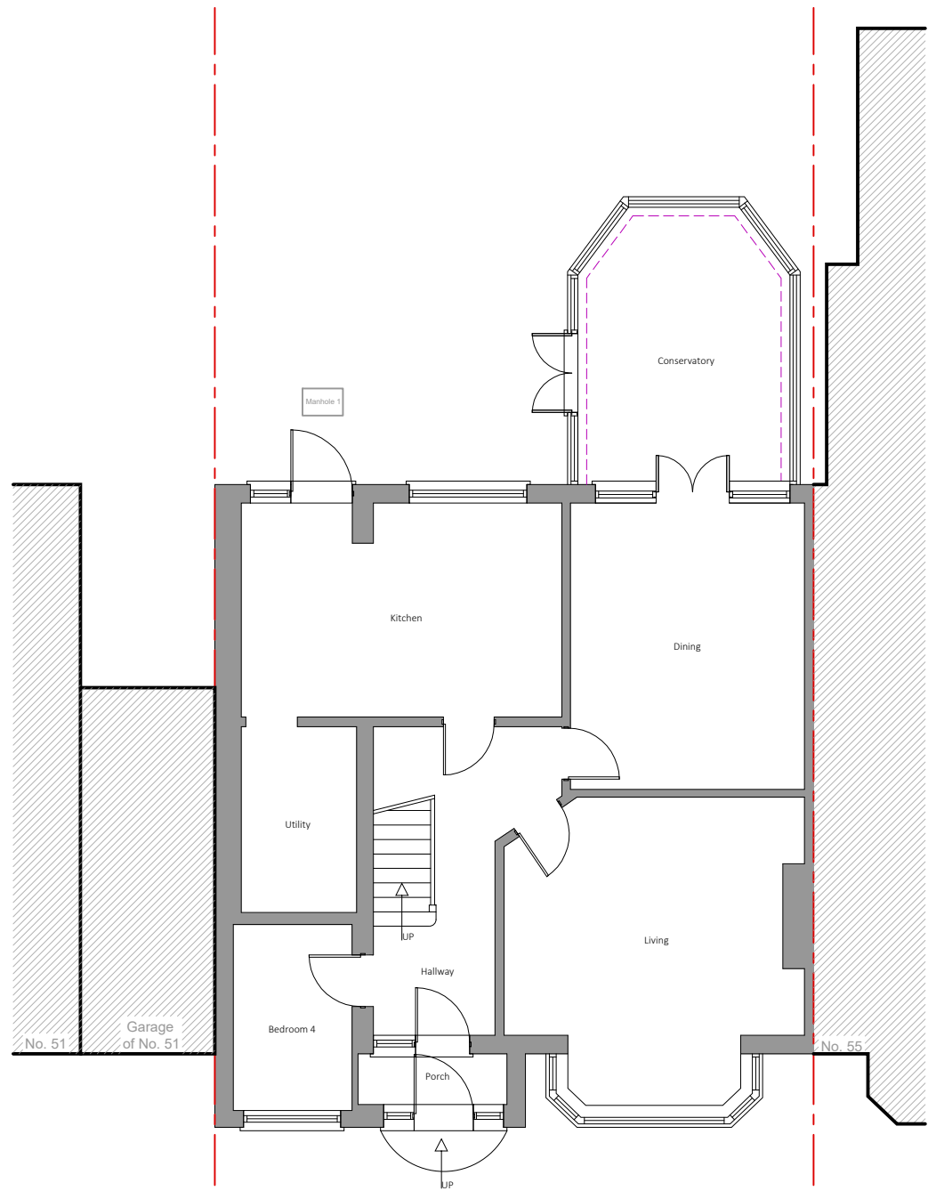
1 Existing Ground Floor Plan
