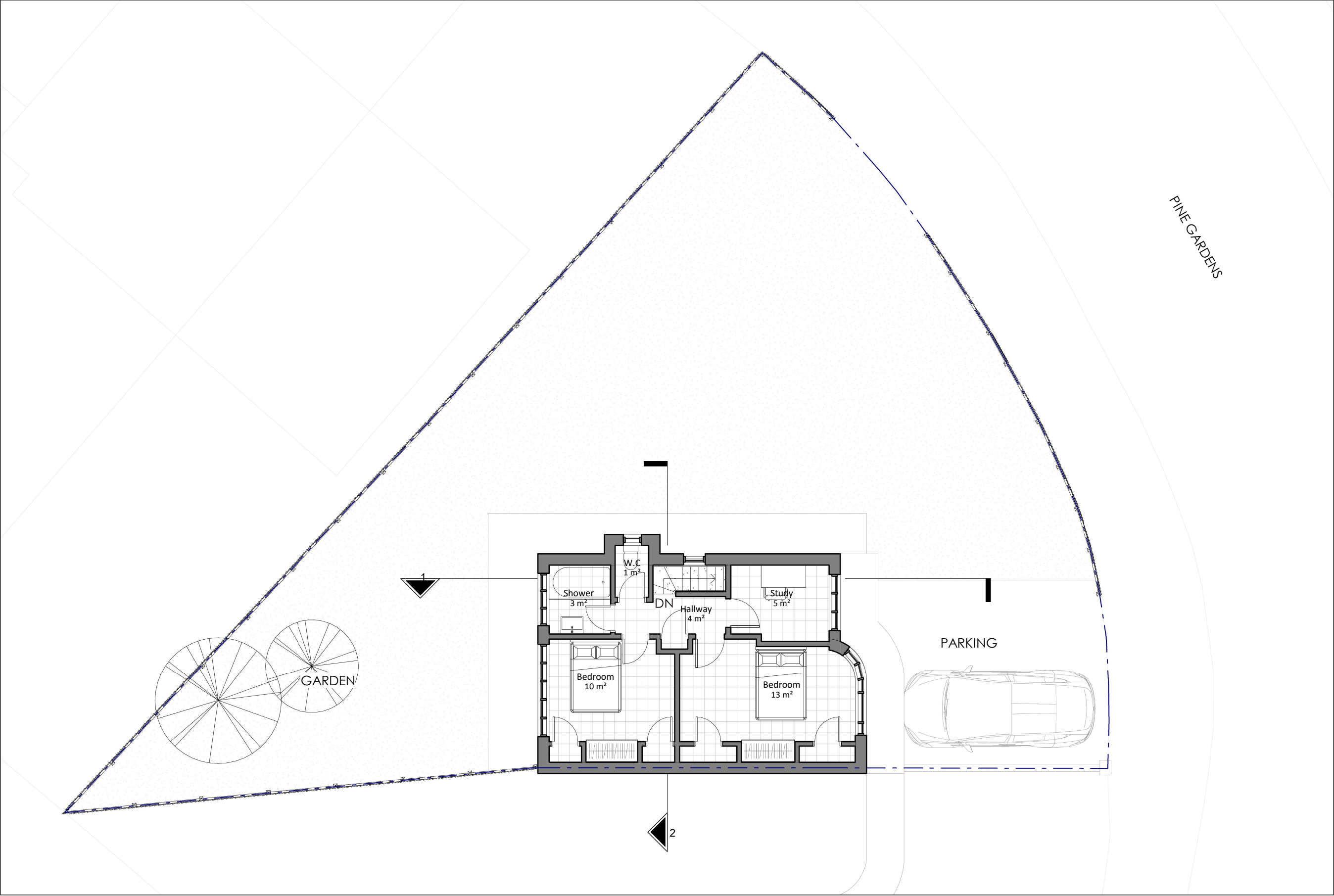
Existing First Floor Plan 1 : 100 0 5m GIA Floor Area : 41.9 m 2
