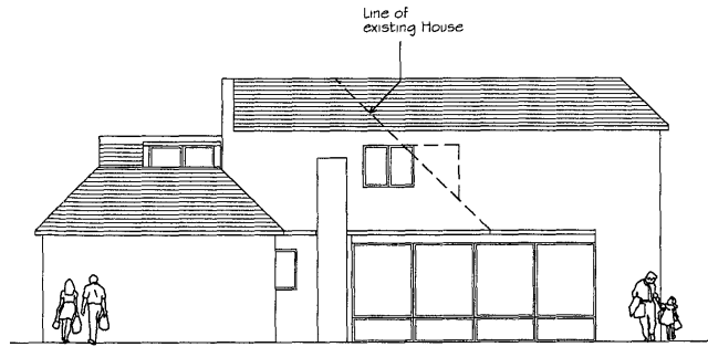
PROPOSED SIDE ELEVATION A-A 1/100
