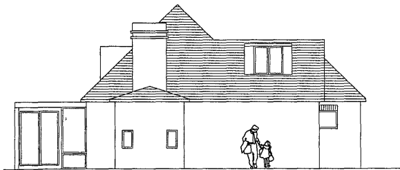
EXISTING SIDE ELEVATION B-B 1/100
