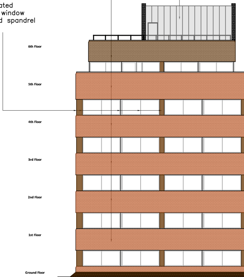
WEST ELEVATION
