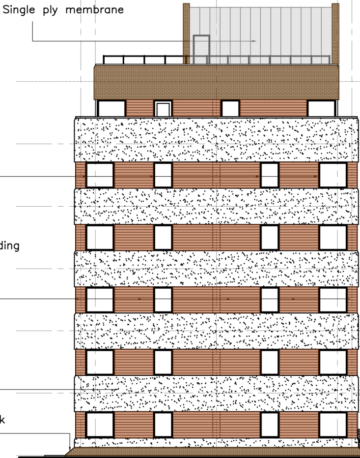
WEST ELEVATION
