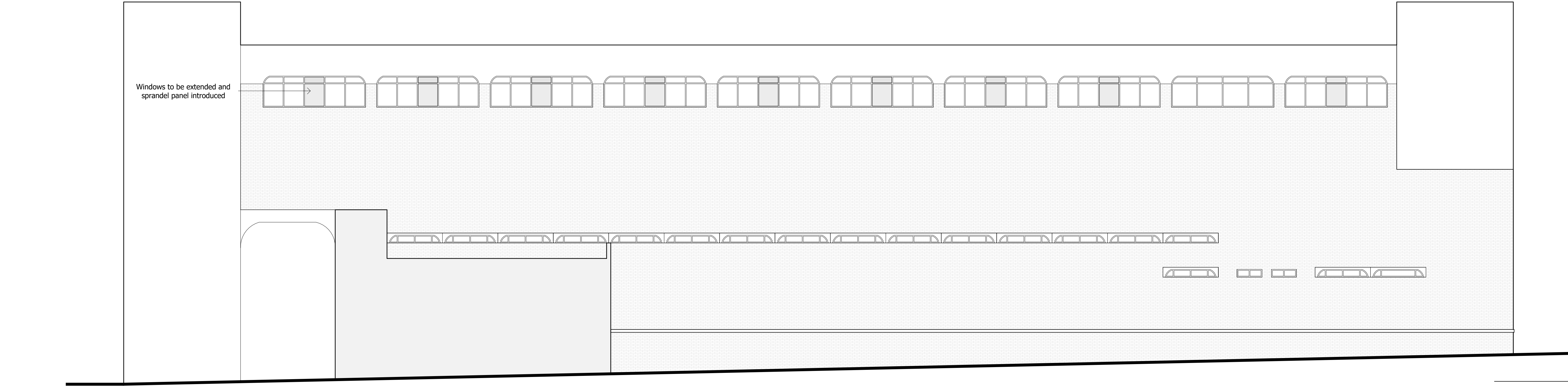
Proposed Elevations 1 : 100
