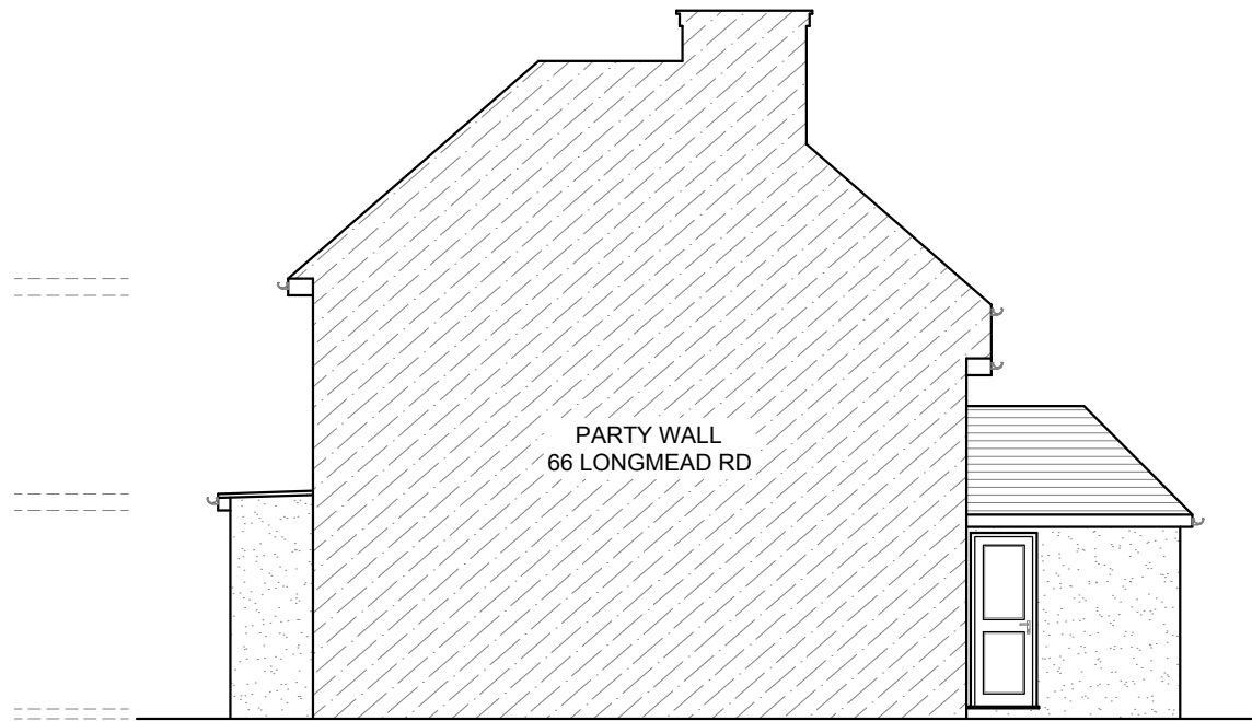
EXISTING SIDE (P#66) ELEVATION SCALE= 1:100
