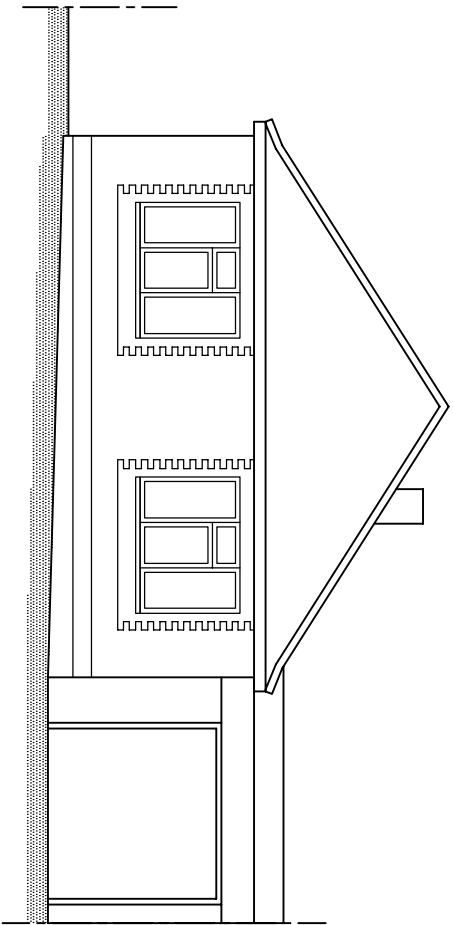
west elevation
