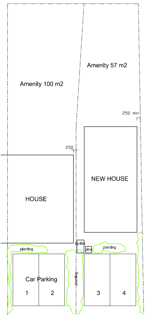
BLOCK PLAN 1:200
