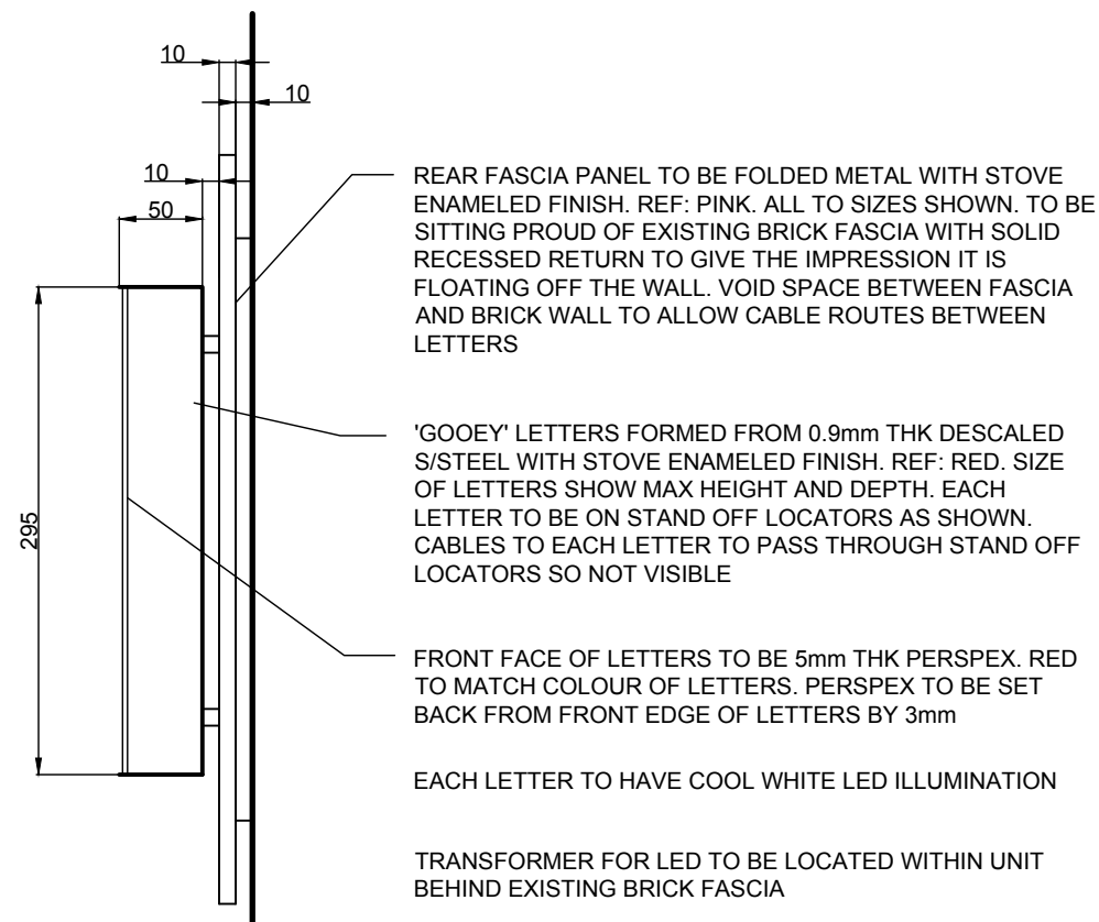
DETAIL one - 1.5
