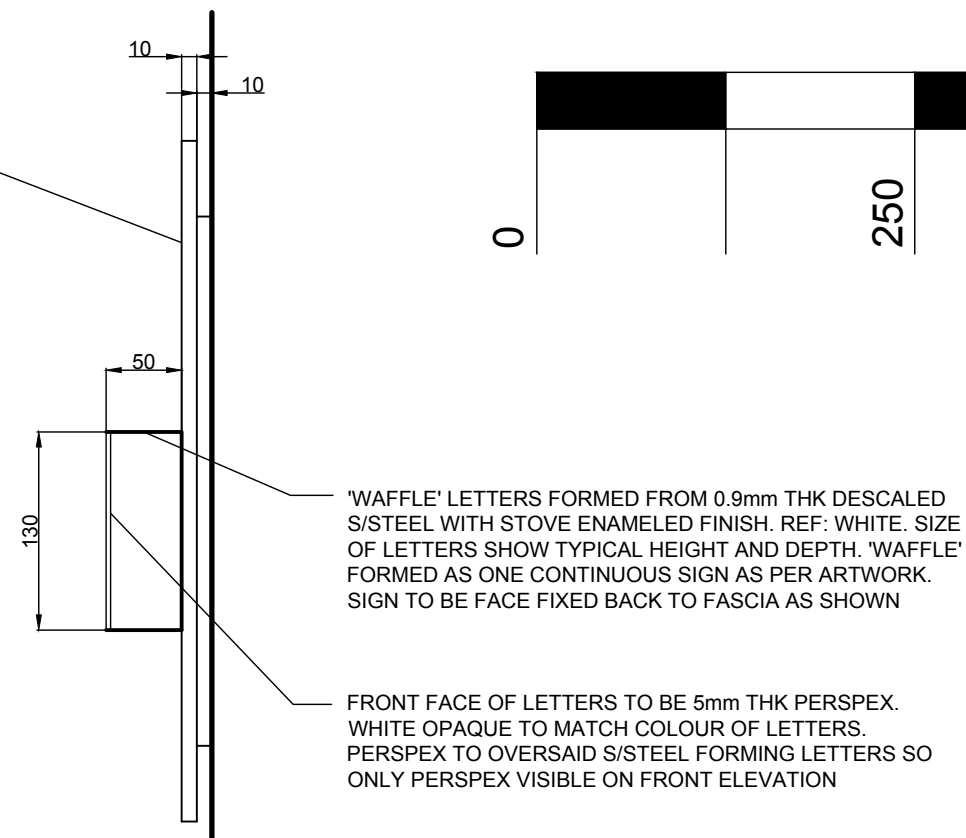
DETAIL two - 1.5
