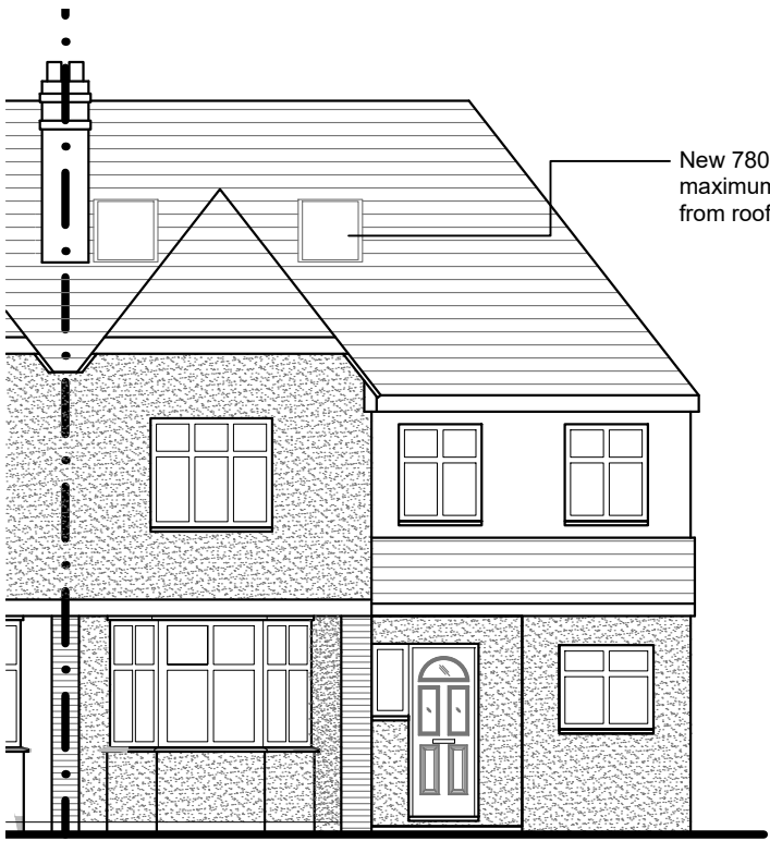
PROPOSED FRONT (SOUTH-EAST) ELEVATION
