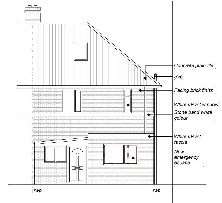
REAR ELEVATION
