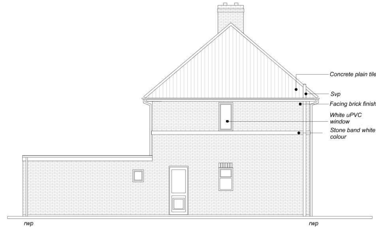
SIDE ELEVATION
