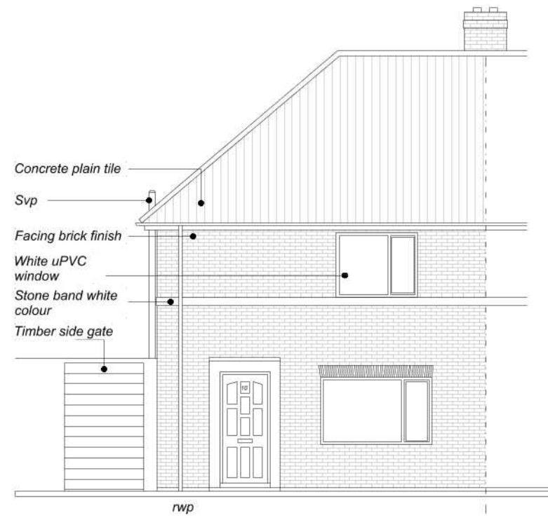
FRONT ELEVATION
