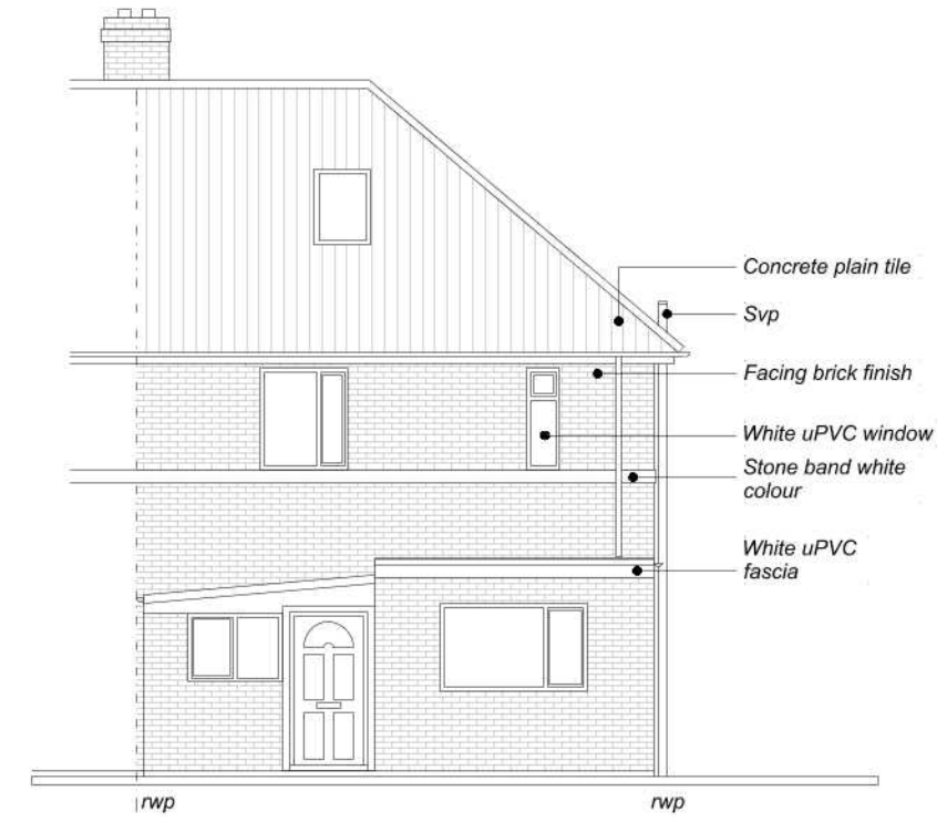
REAR ELEVATION
