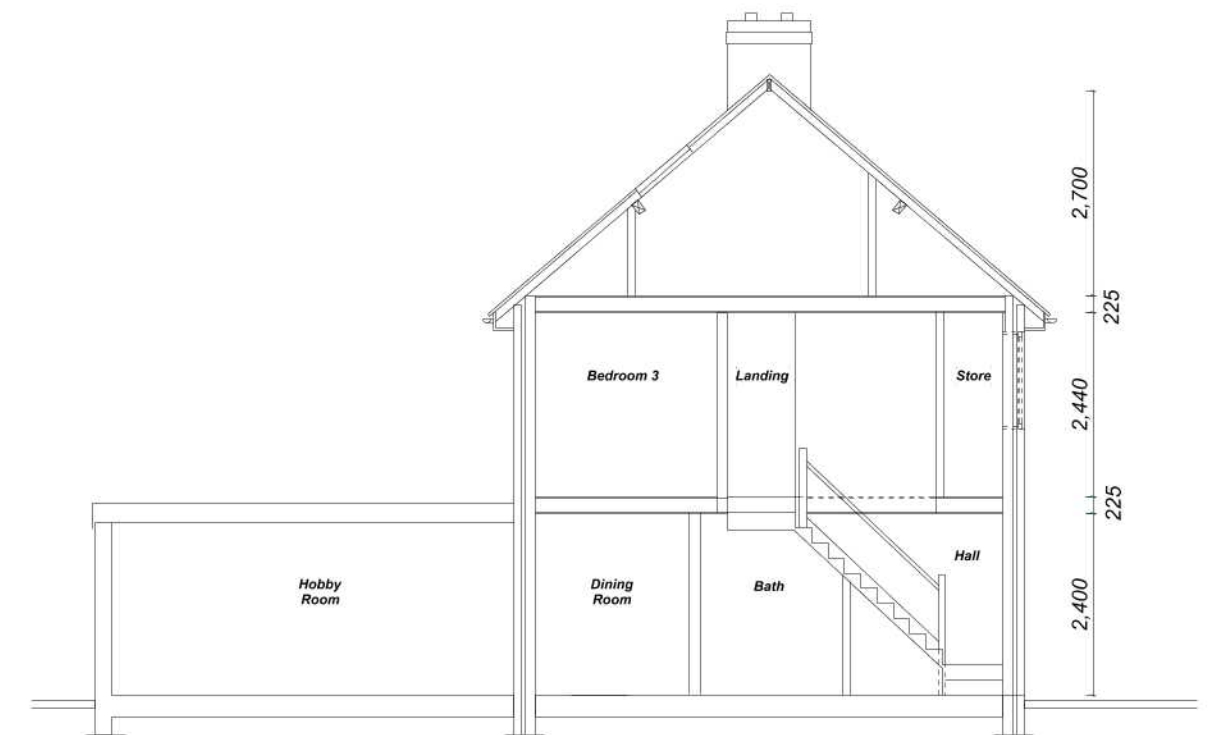
SECTION
