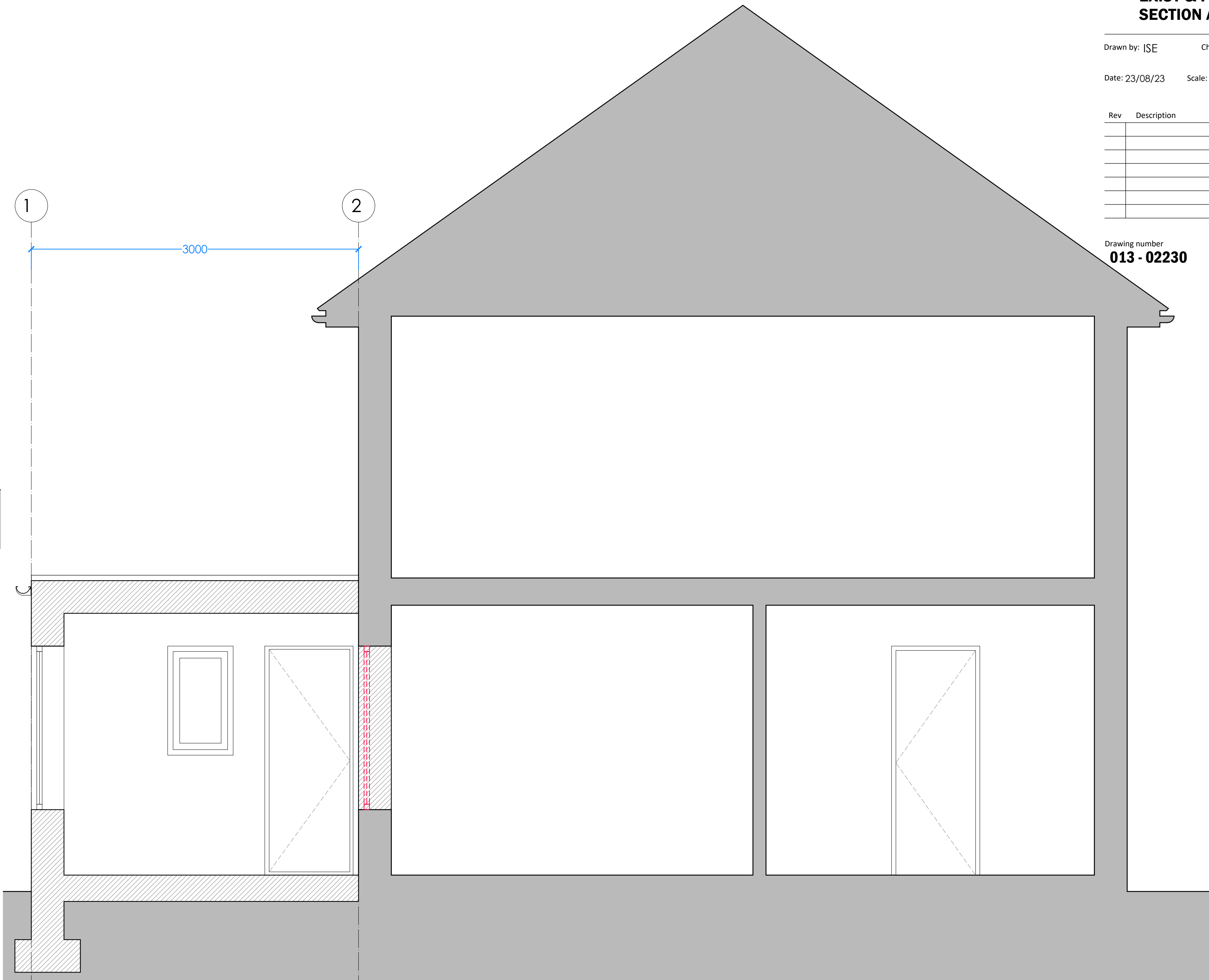
2. PROPOSED SECTION AA 1:25@A1/ 1:50@A3
