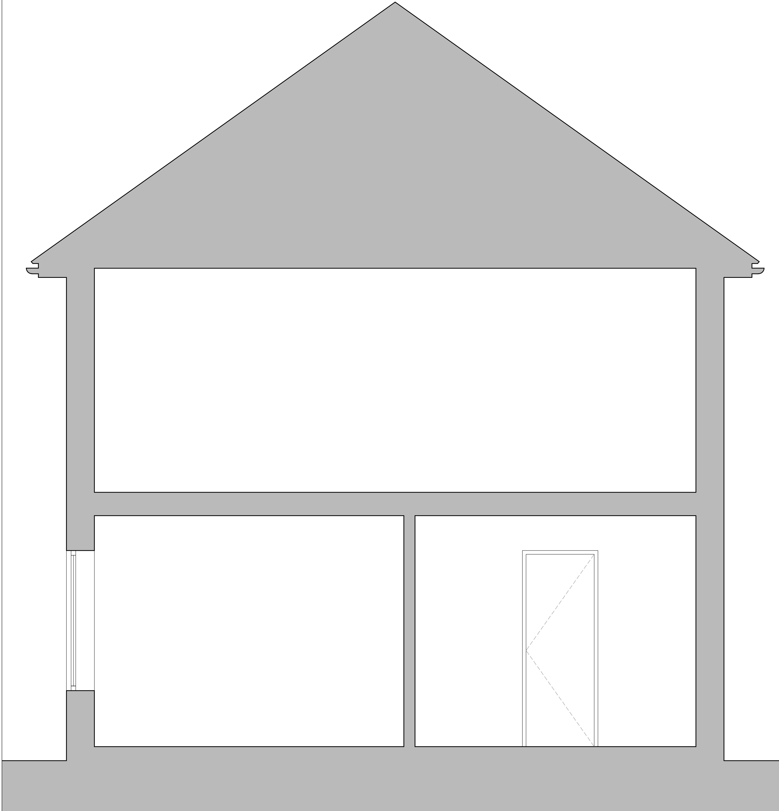
1. EXISTING SECTION AA 1:25@A1/ 1:50@A3
